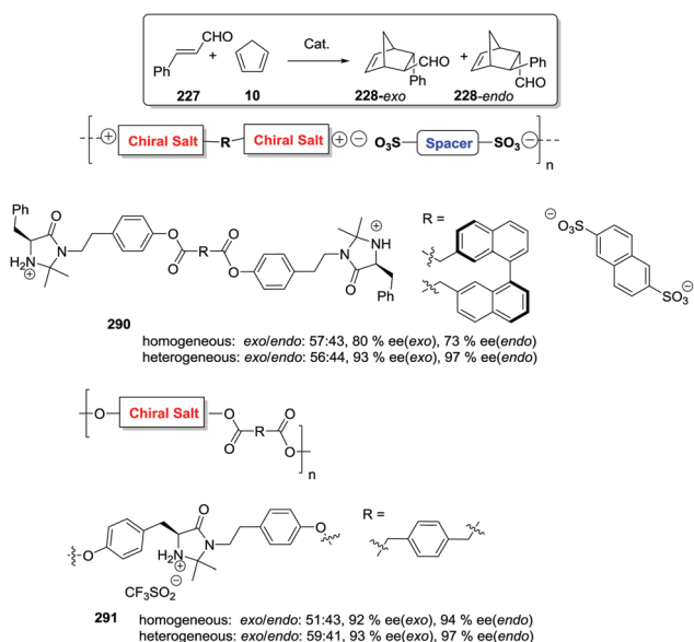
Fig. 72 Preparation of polymer supported ammonium salts derived from MacMillan Imidazolines by polymerization and ion exchange as catalysts for Diels–Alder reaction.
