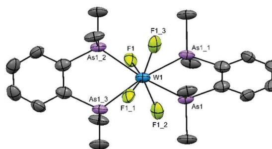
Fig. 2 The cation present in [\text{WF}_4\{\text{o-C}_6\text{H}_4(\text{AsMe}_2)_2\}_2][\text{WF}_8] showing the atom numbering scheme and with ellipsoids drawn at the 50% probability level. Hydrogen atoms are omitted for clarity. Selected bond lengths ( \text{\AA} ) and angles ( ^\circ ): \text{W}(1)\text{-F}(1) = 2.114(6) , \text{W}(1)\text{-As}(1) = 2.6279(10) , \text{As}(1)\text{-W}(1)\text{-As}(1) \#1 = 75.74(4) . Symmetry operators: \#1 = -x + 5/4, -y + 5/4, z ; \#2 = x, -y + 5/4, -z + 1/4 ; \#3 = -x + 5/4, y, -z + 1/4 .
