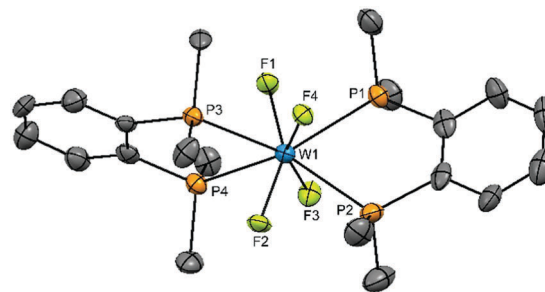
Fig. 1 The cation present in [\text{WF}_4\{\text{o-C}_6\text{H}_4(\text{PMe}_2)_2\}_2][\text{WOF}_5]_2\text{-MeCN} showing the atom numbering scheme and with ellipsoids drawn at the 50% probability level. H atoms are omitted for clarity. Selected bond lengths ( \text{\AA} ) and angles ( ^\circ ): \text{W}(1)\text{-F}(3) = 1.91(4) , \text{W}(1)\text{-F}(2) = 1.92(4) , \text{W}(1)\text{-F}(1) = 1.92(4) , \text{W}(1)\text{-F}(4) = 1.93(4) , \text{W}(1)\text{-P}(3) = 2.572(17) , \text{W}(1)\text{-P}(1) = 2.579(18) , \text{W}(1)\text{-P}(2) = 2.582(18) , \text{W}(1)\text{-P}(4) = 2.592(18) , \text{P}(3)\text{-W}(1)\text{-P}(4) = 72.6(6) , \text{P}(1)\text{-W}(1)\text{-P}(2) = 72.8(6) .
