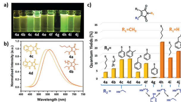
Fig. 2 (a) Solution of ATMs under UV light (365 nm); (b) emission spectra of different alkyl thiol ( 4a–b ) and thiophenol ( 4c–d ) aminomaleimides (recorded at 10 \mu\text{M} in diethyl ether); (c) fluorescence quantum yields of studied ATMs in diethyl ether.
