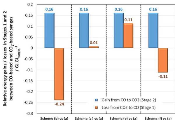
Fig. 14 Relative normalised energy losses in Stage 1 and gains in Stage 2 when (a) methanol and (b) direct DME systems are operated with CO-based and CO 2 -based syngas.
