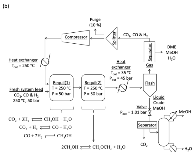
Fig. 4 Schematics of process layouts for direct and indirect DME synthesis from syngas.
