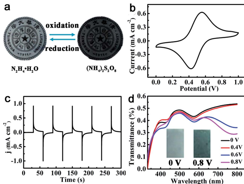
Fig. 3 Responsive properties of ACAT-vitrimer to redox chemicals and voltages. (a) Chemical redox response of ACAT-vitrimer. (b) Cyclic voltammogram curve of ACAT-vitrimer on FTO conducting glass measured in 0.5 M \text{H}_2\text{SO}_4 (a solution of \text{H}_2\text{O} and DMSO) at a scan rate of 50 \text{ mV s}^{-1} . (c) Chronoamperometry curves when the anodic potential was switched between 0 V and 0.8 V (vs. Ag/AgCl) for 30 s at each step. (d) Transmittance spectra of ACAT-vitrimer film under different applied potentials in the range of 0 V to 0.8 V (vs. Ag/AgCl) for 30 s at each potential (inset: photographs of ACAT-vitrimer at voltages of 0 V and 0.8 V).
