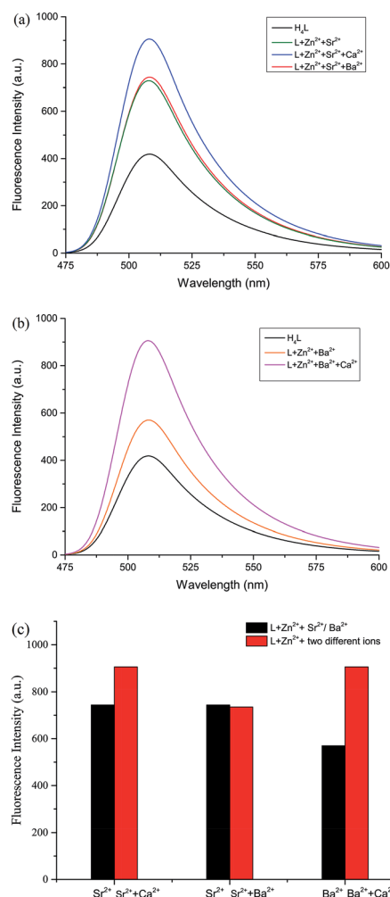
Fig. 6 (a) Fluorescence spectra of complex 2 solution ( 1.0 \times 10^{-5} \text{ mol L}^{-1} ) in the absence and presence of various metal ions (1.0 equiv. of Ca(II) and Ba(II)). (b) Fluorescence spectra of complex 3 solution ( 1.0 \times 10^{-5} \text{ mol L}^{-1} ) in the absence and presence of various metal ions (1.0 equiv. of Ca(II)). (c) Fluorescence response of L–Zn(II) solution ( 1.0 \times 10^{-5} \text{ mol L}^{-1} ) to various metal ions. ex = 367 nm, em = 508 nm.
