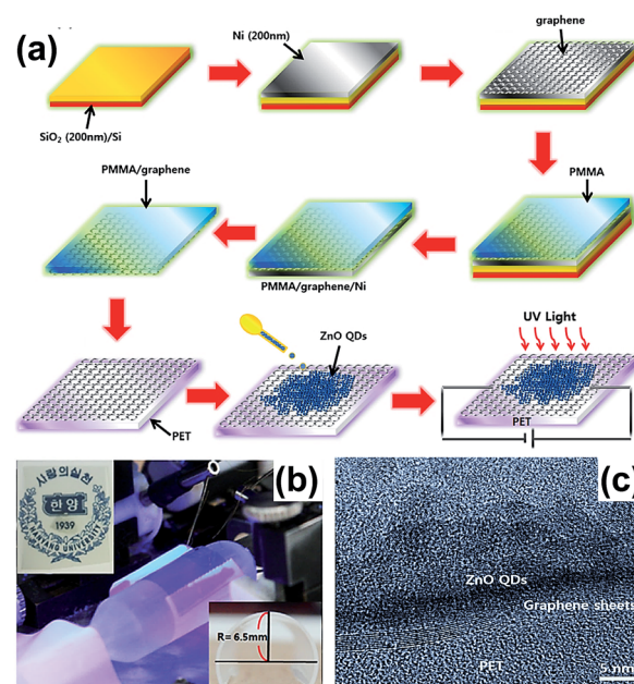
Fig. 7 (a) Illustration of the preparation of the ZnO cQDs/GR composite. (b) Images of the equipment and device; the inset on the bottom right shows a flexible UV photodetector. (c) HRTEM image of the ZnO cQDs/GR composite on a polyethylene terephthalate (PET) substrate. Reprinted with permission from ref. 58. Copyright 2015 Elsevier Ltd.
