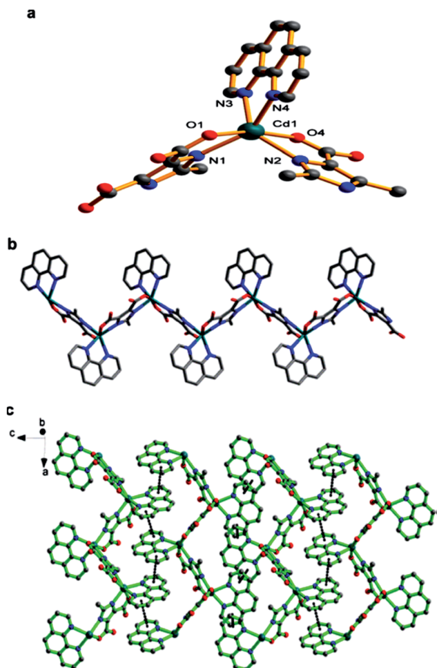
Fig. 15 (a) Molecular square structure of CP with [Cd(HL)(phen)]_n unit based on 2-ethyl-1H-imidazole-4,5-dicarboxylic acid. (b) 1D chain of CP. (c) 2D sheet of CP supported by \pi - \pi stacking interactions. [Reprinted from ref. 158 Copyright 2012, with permission from Elsevier.]
