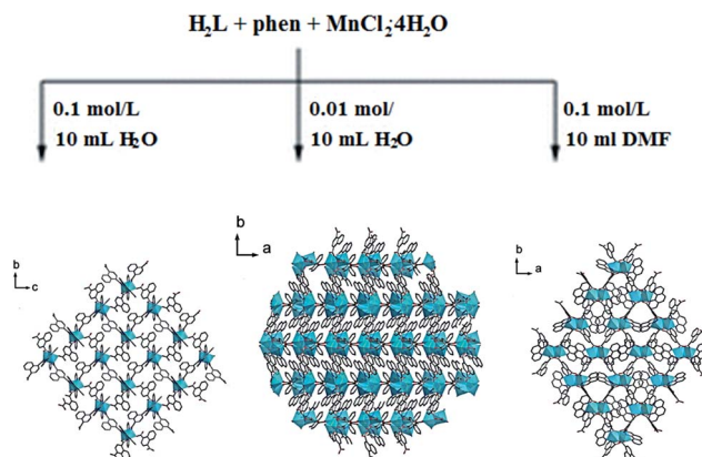
Scheme 13 The formation of various crystal structures in different solvents and concentrations during interaction of 1,4-naphthalene dicarboxylic acid, phen and MnCl_2 . [Reproduced from ref. 159 with permission from The Royal Society of Chemistry.]
