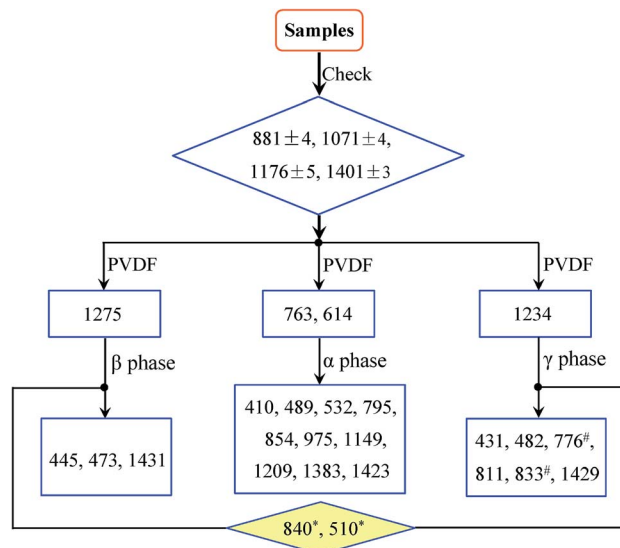
Fig. 1 Flow diagram for the identification of \alpha , \beta and \gamma phases; 840* and 510* represents bands in the range of 837–841 and 508–512 cm -1 , respectively; 776# and 833# reflects possible variations based on specific processes.
