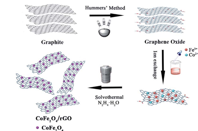
Scheme 1 Schematic of the in situ synthetic route for the CFG nanocomposites.
