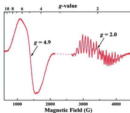
Fig. 18 EPR spectrum of the oxidized Mn(IV) 3 Mn(III) form ( S_2 -state) of the synthetic complex by Zhang et al. at 7 K 197 (from Zhang et al. , Science , 2015, 348 , 690. Reprinted with permission from AAAS.).
