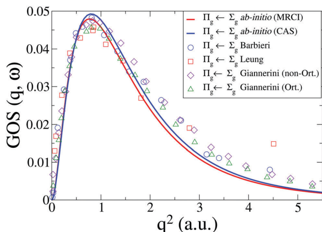
Fig. 7 Generalized oscillator strength, GOS(q, \omega) , for the a^1\Pi_g \leftarrow X^1\Sigma_g^+ transition in N_2 . Our CASSCF and MRCI ab initio results are compared to experimental results from Leung et al. 42 and Barbieri et al. , 64 and to calculations by Giannerini et al. 65
