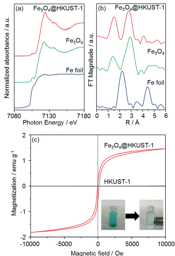
Fig. 5 Fe K-edge (a) XANES and (b) FT-EXAFS spectra of \text{Fe}_3\text{O}_4 , \text{Fe}_3\text{O}_4@HKUST-1 and Fe metallic foil. (c) Magnetization curves of \text{Fe}_3\text{O}_4@HKUST-1 and HKUST-1, and photographs of \text{Fe}_3\text{O}_4@HKUST-1 collected by a magnet. The magnetization measurements were performed at 300 K.
