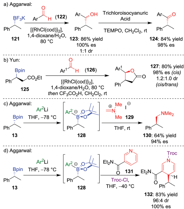
Scheme 18 Additions of trifluoroborate salts and boronate complexes to aldehydes and iminium ions. Ar = p - \text{CF}_3\text{C}_6\text{H}_4 , Ar 1 = p - \text{NO}_2\text{C}_6\text{H}_4 , Ar 2 = 3,5-( \text{CF}_3 ) 2 \text{C}_6\text{H}_3 , Troc-Cl = 2,2,2-trichloroethyl chloroformate.
