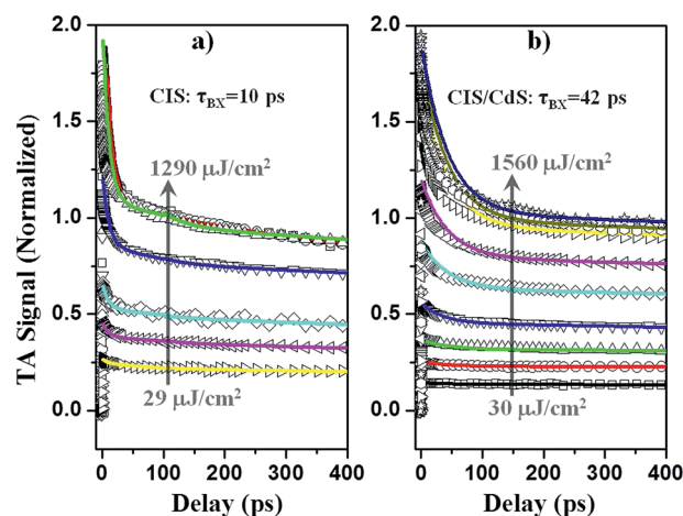
Fig. 5 Normalized exciton bleach TA kinetics (open symbols) at different excitation intensities for (a) CuInS 2 core, and (b) CuInS 2 /CdS core/shell QDs. The solid lines are fits to a multicarrier annihilation model described in the main text.
