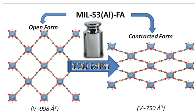
Fig. 1 Schematic representation of the pressure-induced contraction of MIL-53(Al)-FA between an open and a contracted form.
