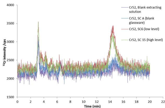
Fig. 6 HPLC-ICP-MS chromatogram of Cr species in mainstream smoke from cigarette spiked two different spike levels (5.80 and 9.80 \mu g g -1 of chromium, respectively) using 2.8 mM TPABr and 4 mM EDTA (pH 8.5) as extractant. 0.18 mM, 1 mM EDTA (pH 8) as mobile phase at a flow rate of 0.8 mL min -1 .
