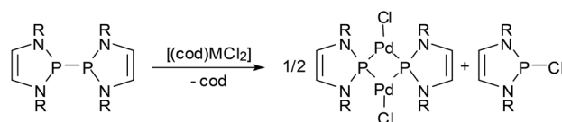
Scheme 15 (a) Reduction of complex group-10 metal dihalides ( \text{M} = \text{Pd}, \text{Pt} ) with a bis-diazaphospholenyl to phosphonium-metal(0)-halides ( \text{R} = \text{Dipp} ).
