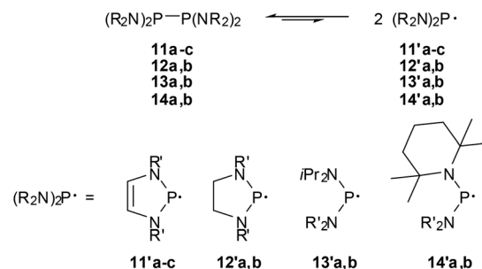
Scheme 13 P–P bond dissociation equilibria for tetraamino-diphosphines (R' = t Bu ( 11a ), 2,6-Me 2 C 6 H 3 ( 11b ), 2,6- i Pr 2 C 6 H 3 ( 11b , 12a ), 2- t Bu 2 C 6 H 4 ( 12b ), i Pr ( 13a , 14b ), SiMe 3 ( 13b ), Et ( 14a )).
