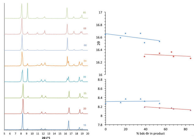
Fig. 3 PXRD patterns of the compounds [\text{Zn}_2(\text{bdc})_{2-x}(\text{bdc-Br})_x(\text{dabco})] \cdot n\text{DMF} 1 , with the number shown against each powder pattern denoting the % bdc-Br in the sample. The plot of 2\theta against % bdc-Br shows the key peaks which shift with the change in pore topology.
