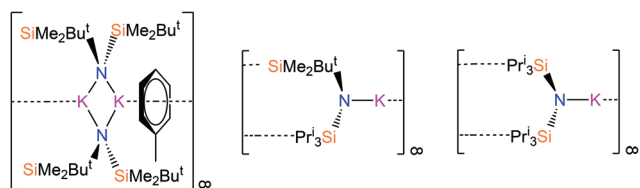
Fig. 1 The potassium silylamide complexes [\{\text{K}[\mu\text{-N}(\text{SiMe}_2\text{Bu}^t)_2]\}_2(\text{C}_7\text{H}_8)]_\infty , [\text{K}\{\text{N}(\text{SiPr}^i)_3\}(\text{SiMe}_2\text{Bu}^t)]_\infty and [\text{K}\{\text{N}(\text{SiPr}^i)_2\}]_\infty . 28
