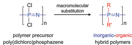
Fig. 1 Generic structure of poly(organo)phosphazenes, a family of molecular hybrid polymers, most-commonly prepared from the precursor poly(dichloro)phosphazene [\text{N}(\text{P}(\text{Cl})_2)_n] .
