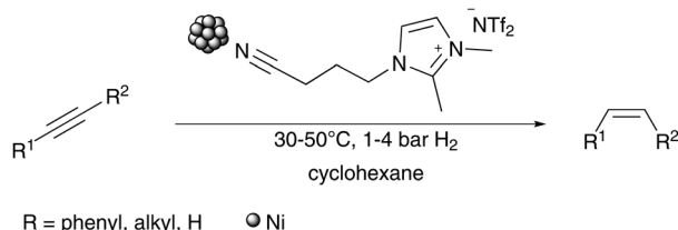
Scheme 1 Semihydrogenation of alkynes using Ni-NPs in nitrile functionalised IL.
