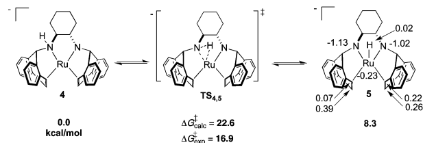
Scheme 3 DFT calculated free energies (relative to 4 ) for proposed N–H addition/elimination reactions in solution. Energies are presented in \text{kcal mol}^{-1} and APT charges in ESU are also shown for 5 .
