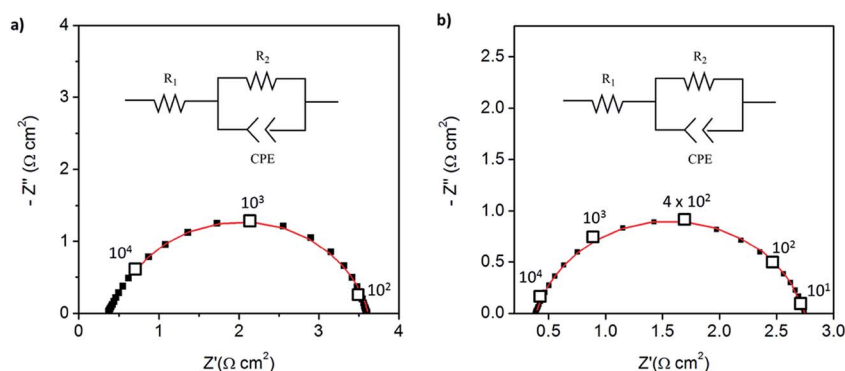
Fig. 6 Symmetric cell impedance measurements of 30 wt% Pt-CNT based electrodes prepared by (a) strategy 1 (see Scheme 2) in which Pt-CNT bearing and CDP bearing solutions were electro sprayed sequentially, and (b) strategy 2 in which a single Pt-CNT and CDP bearing solution was sprayed. In (a), the Pt loading and utilization are 4.2 \times 10^{-3} \text{ mg cm}^{-2} Pt and 64 \text{ S mg}^{-1} , respectively, whereas in (b) they are 5.1 \times 10^{-3} \text{ mg cm}^{-2} Pt and 86 \text{ S mg}^{-1} . Measurements are performed at 240^\circ\text{C} in a dynamic atmosphere of 0.4 \text{ atm H}_2\text{O} and balance \text{H}_2 supplied at a gas velocity of 6 \text{ cm min}^{-1} and spectra are taken after 4 hours (insets: equivalent circuit used for fitting).
