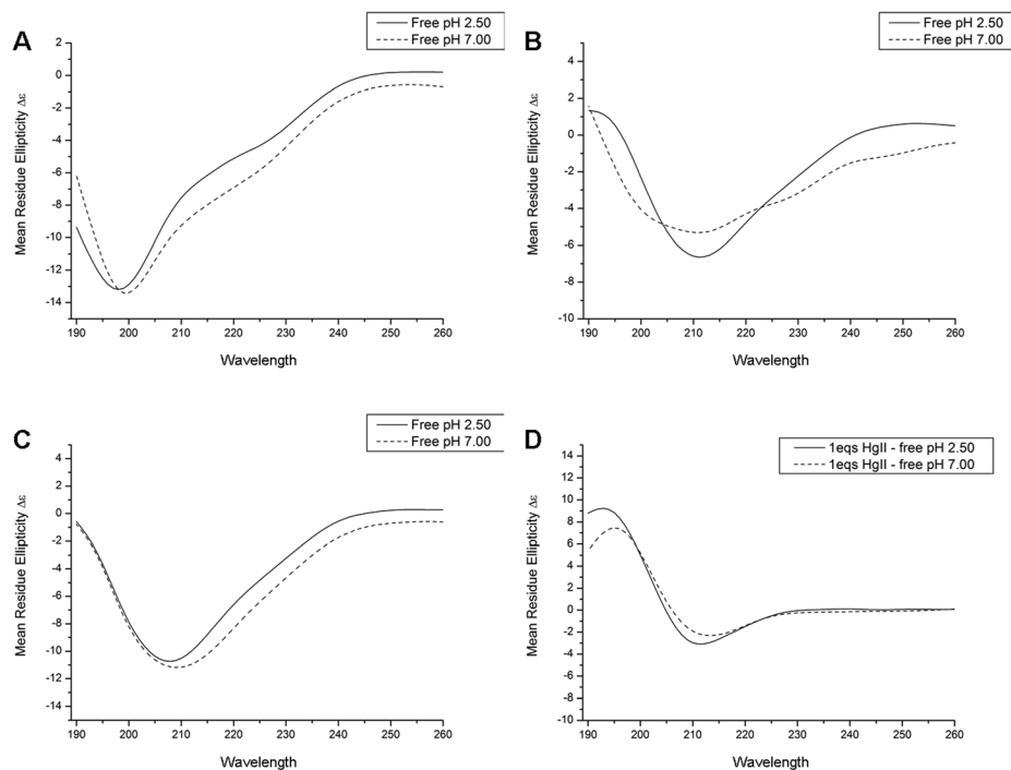
Fig. 4 CD spectra recorded at pH 2.5 (3 mM HCl) and 7.0 (50 mM phosphate buffer) for 10 μM apo Bri2-23 (A), 10 μM Bri2-23 in presence of 1.0 equivalent of Ag(I) (B), 10 μM Bri2-23 in presence of 1.0 equivalent of Hg(II) (C) and difference CD spectra for mercurated peptide and its apo form (D).
