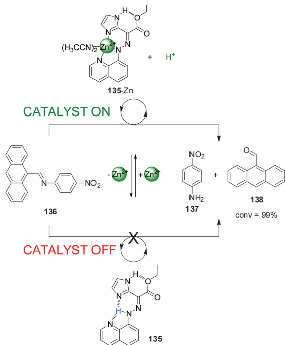
Scheme 37 Controlling the hydrolysis of imine 136 by switchable \text{H}^+ capture/release through coordination of 135 to \text{Zn}^{2+} . 68
