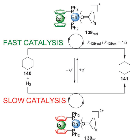
Scheme 38 \text{Co}^{(II)}/\text{Co}^{(III)} redox control over the activity of a Rh(I) hydrogenation catalyst 139 . 69
