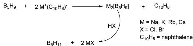
Scheme 28 Preparation of dianion (B 5 H 9 ) 2- and B 5 H 11 .
