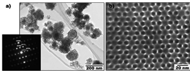
Fig. 7 TEM images at low (a) and high (b) magnifications of KIT-6 mesoporous \text{Co}_3\text{O}_4 , showing highly ordered mesopores. The inset is the corresponding SAED pattern of the circled zone. Reprinted with permission from ref. 72. Copyright 2010, Wiley-VCH.
