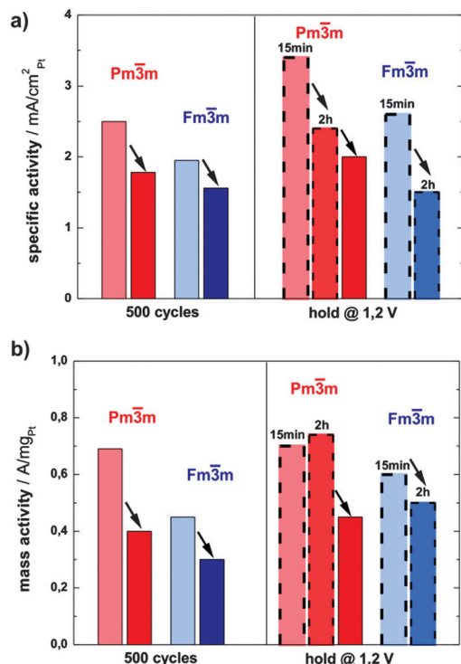
Fig. 4 Comparison of (a) specific and (b) mass activities @ 0.9 V RHE of the ordered (red) and the disordered (blue) catalysts after dealloying (500 cycles and potential hold @ 1.2 V for 15 min and 2 hours, respectively) and subsequent degradation (dark red and dark blue color). No subsequent degradation after holding the potential at 1.2 V RHE was done for the disordered catalyst.
