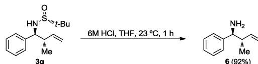
Scheme 2 Desulfurination of 3q .
