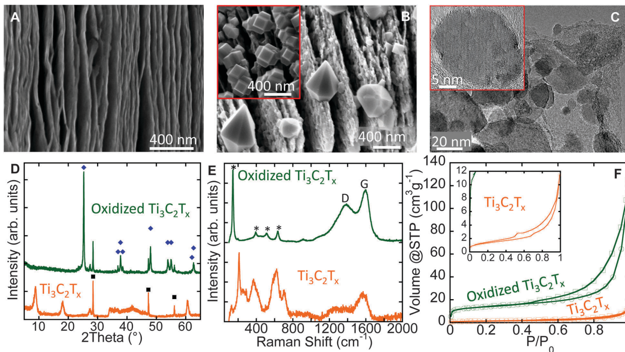
Fig. 2 Characterization of \text{Ti}_3\text{C}_2\text{T}_x powders before and after flash oxidation in air at 1150^\circ\text{C} for 30 s. (A) SEM image of typical as-synthesized multilayers \text{Ti}_3\text{C}_2\text{T}_x . (B) SEM image after oxidation. Top left inset is another SEM image at a different location for the same sample. (C) TEM image after oxidation. Inset is a high-magnification image of one of the anatase particles embedded in the amorphous carbon. (D) XRD patterns before and after oxidation. The blue diamonds denote anatase peak positions for (PDF#01-0562); squares denote Si peak positions which was used as an internal reference. (E) Raman spectra before and after oxidation; the stars represent anatase; D and G represent the positions of D and G bands of disordered graphitic carbon. (F) Nitrogen adsorption-desorption isotherms at -196^\circ\text{C} for \text{Ti}_3\text{C}_2\text{T}_x before and after oxidation. The inset shows a zoom of the \text{Ti}_3\text{C}_2\text{T}_x isotherms along the Y-axis.
