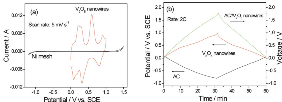
Fig. 12 (a) CV curve of \text{V}_2\text{O}_5 nanowires and Ni mesh (current collector) and (b) charge/discharge curves of AC// \text{V}_2\text{O}_5 nanowires in 0.5\text{ mol l}^{-1} \text{K}_2\text{SO}_4 aqueous solution (modified from ref. 6a).
