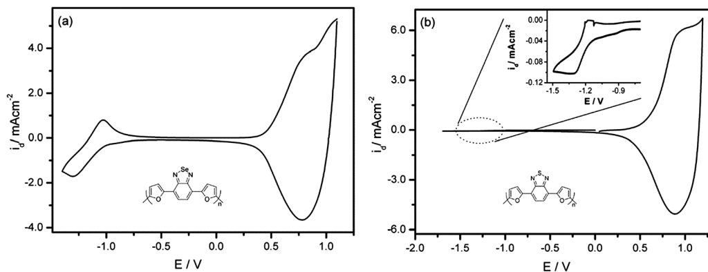
Fig. 5 Cyclic voltammograms of (a) PFSeF and (b) PFSF in 0.1 M TBAH/ACN electrolyte solution at a scan rate of 100 \text{ mV s}^{-1} vs. Ag/AgCl.
