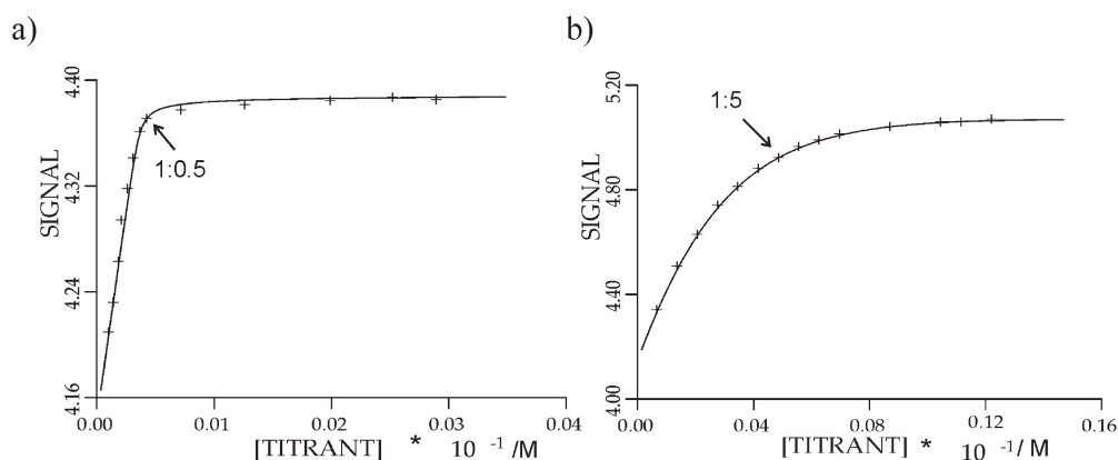
Fig. 6 Plot of the observed (×) and calculated (–) chemical shifts of the NH resonances of 27 (1.02 mM) as a function of added \beta -maltoside 28 (a) or \beta -glucopyranoside 2a (b). The [receptor]:[sugar] ratio is marked. 24
