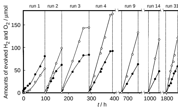
Fig. 1 Time courses of H 2 (open circles) and O 2 (filled circles) evolution in Cu 2 O under visible light (λ ≥ 460 nm) irradiation. Catalyst: 0.5 g, H 2 O: 200 cm 3 . The reaction system was evacuated with light irradiation after each run. Time courses in runs 5–8, 10–13 and 15–30 are omitted.
