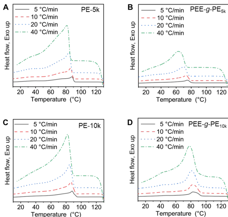
Figure 8. DSC curves during non-isothermal crystallization at different cooling rates for (A) PE-5k, (B) PEE- g -PE 5k , (C) PE-10k, and (D) PEE- g -PE 10k .
