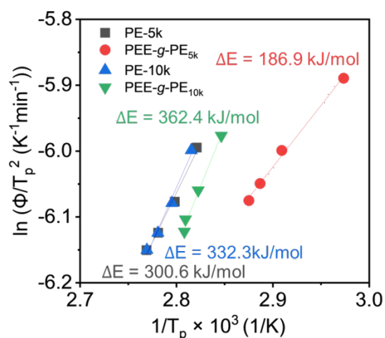
Figure 11. Plots of \ln\left(\frac{\phi}{T_p^2}\right) versus \frac{1}{T_p} for PE-5k, PEE- g -PE 5k , PE-10k, and PEE- g -PE 10k .
