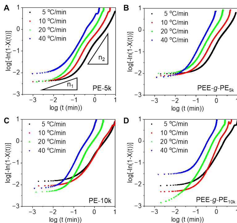
Figure 9. Plots of \log[-\ln(1-X(t))] versus \log t for non-isothermal crystallization of (A) PE-5k, (B) PEE-g-PE 5k , (C) PE-10k, and (D) PEE-g-PE 10k .
