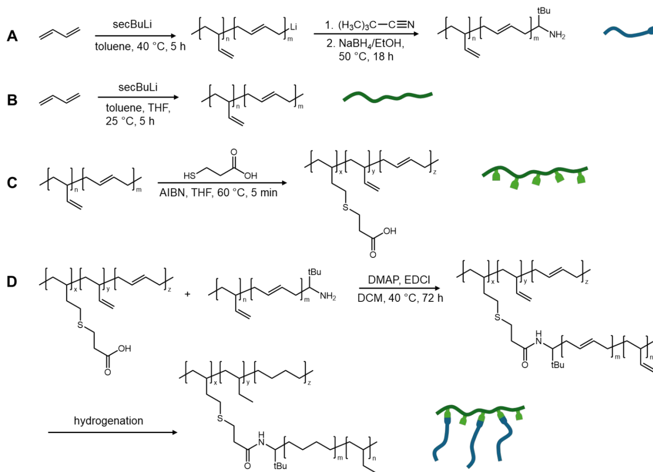
Figure 1 Reaction scheme of (A) amine-terminated 1,4-PB, n/(m+n)=0.12 ; (B) 1,2-PB, n/(m+n)=0.89 ; (C) carboxyl functionalized 1,2-PB, and (D) polyethylethylene-graft-polyethylene.
