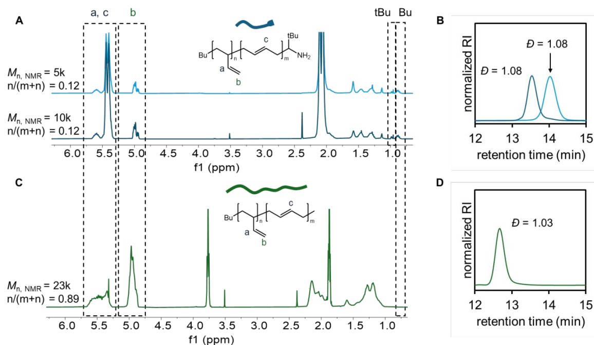
Figure 2 (A) ^1\text{H} NMR spectra of 1,4-PB-NH 2 graft, (B) GPC result of 1,4-PB-NH 2 graft, (C) ^1\text{H} NMR spectrum of 1,2-PB backbone, and (D) GPC result of ^1\text{H} NMR of 1,2-PB backbone.
