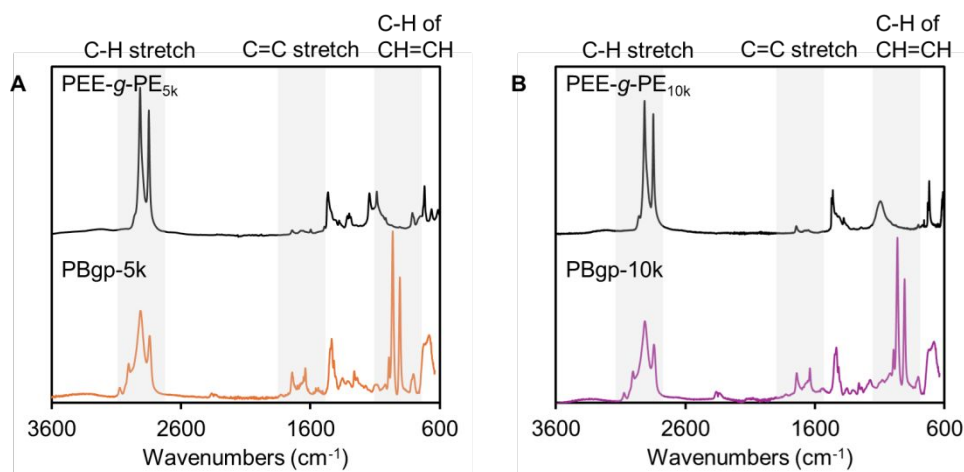
Figure 6. FTIR of (A) PBgp-5k and the hydrogenated polymer PEE- g -PE 5k , and (B) PBgp-10k and the hydrogenated polymer PEE- g -PE 10k .
