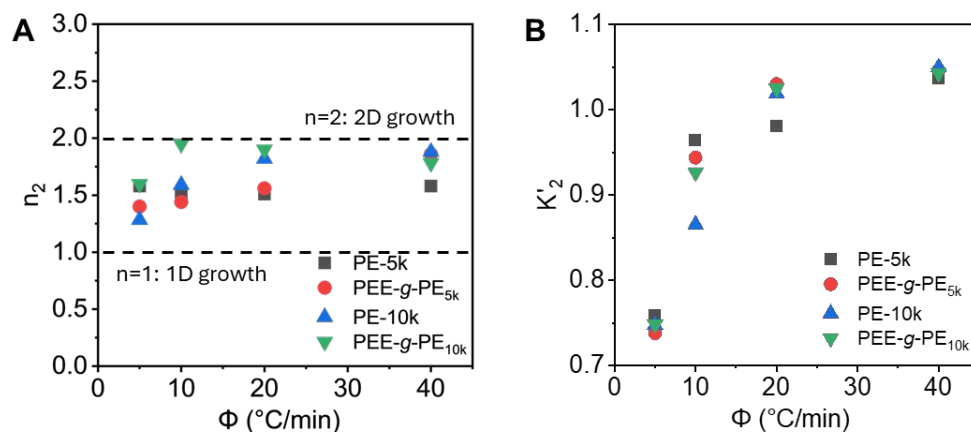
Figure 10. (A) Avrami exponent and (B) Jeziorny-modified Avrami constant for non-isothermal crystallization of PE-5k, PEE-g-PE 5k , PE-10k, and PEE-g-PE 10k .
