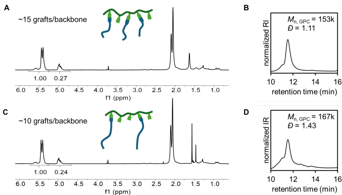
Figure 5 (A) 1 H NMR of the isolated PBgp-5k, (B) GPC trace of the isolated PBgp-5k, (C) 1 H NMR of the isolated PBgp-10k, and (D) GPC trace of the isolated PBgp-10k.
