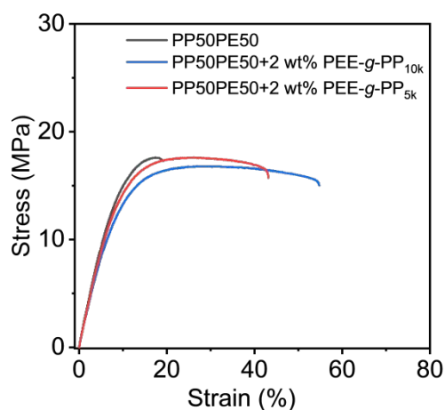
Figure 12. Representative stress–strain curves for LDPE:iPP (50:50) blends with and without 2 wt% graft copolymer PEE-g-PEs.
