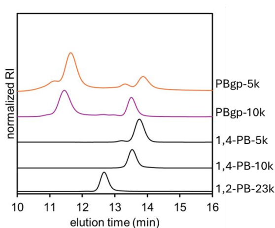
Figure 4. GPC traces of the backbone PB (1,2-PB-23k), 1,4-PB grafts (1,4-PB-5k and 1,4-PB-10k), the product from the coupling reaction with 5k graft (PBgp-5k) and 10k graft (PBgp-10k).
