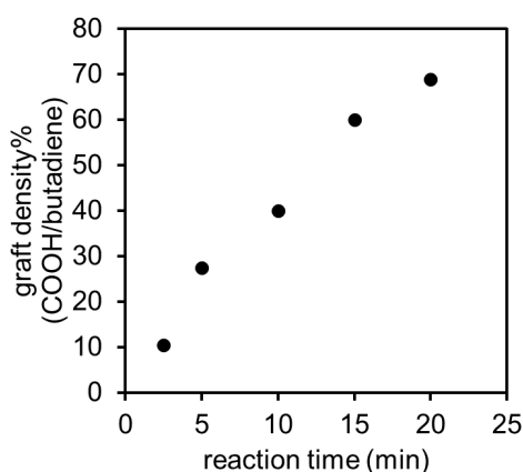
Figure 3. Effect of reaction time on the grafting density of the carboxyl functionalization of 1,2-PB
