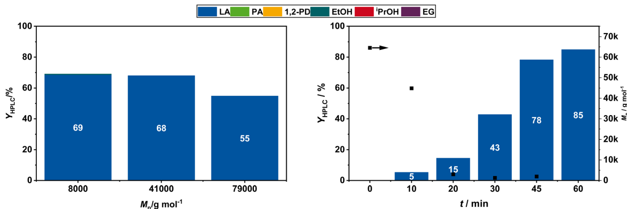
Fig. 1 Chemical recycling results for (left) PLA with different molecular weights ranging from 8000 to 79 000 \text{g mol}^{-1} . Conditions: 5 mg \text{Ru}_5 \text{ wt\%/CeO}_2 , 115 mg PLA, 175 ^\circ\text{C} , 5 bar \text{H}_2 , 5 mL \text{H}_2\text{O} , 500 rpm, 0.5 h, 50 mL Hastelloy autoclave. (right) PLA after different reaction times ranging from 0 to 60 min. Black squares are attributed to the right y-axis M_n . Conditions: 5 mg \text{Ru}_5 \text{ wt\%/CeO}_2 , 115 mg PLA, 175 ^\circ\text{C} , 5 bar \text{H}_2 , 5 mL \text{H}_2\text{O} , 500 rpm, 0–1 h, 50 mL Hastelloy autoclave. Abbreviations: LA – lactic acid, PA – propionic acid, 1,2-PD – propionic acid, EtOH – ethanol, iPrOH – isopropanol, EG – ethylene glycol. Note: Species listed in the legend other than lactic acid (LA) were not detected under the applied conditions. They are included as potential degradation products for completeness.
