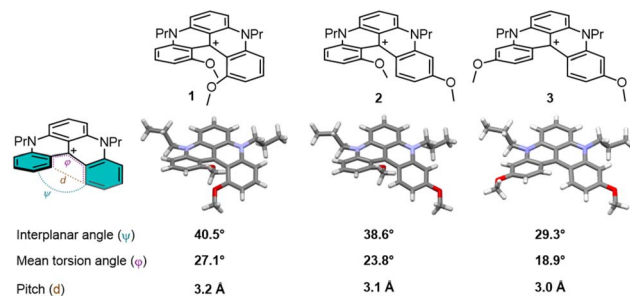
Fig. 2 Selected structural features of DMQA 1 , 2 and 3 .
