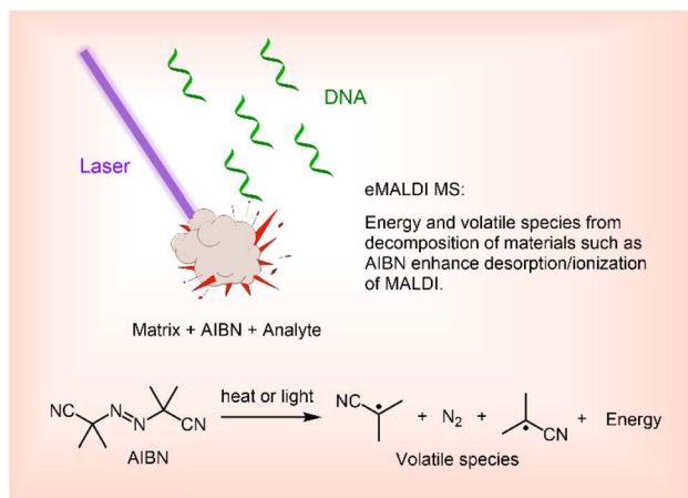
Fig. 1 The concept of enhanced MALDI MS (eMALDI MS).
