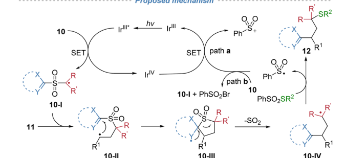
Scheme 5 Polarity-umpolung three-component radical alkylation of alkenes.
