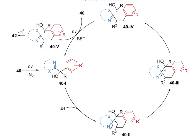
Scheme 15 Radical-mediated 1,2-arylheteroarylation of alkenes with tertiary alcohol-based aryldiazonium salts as bifunctional reagents.
