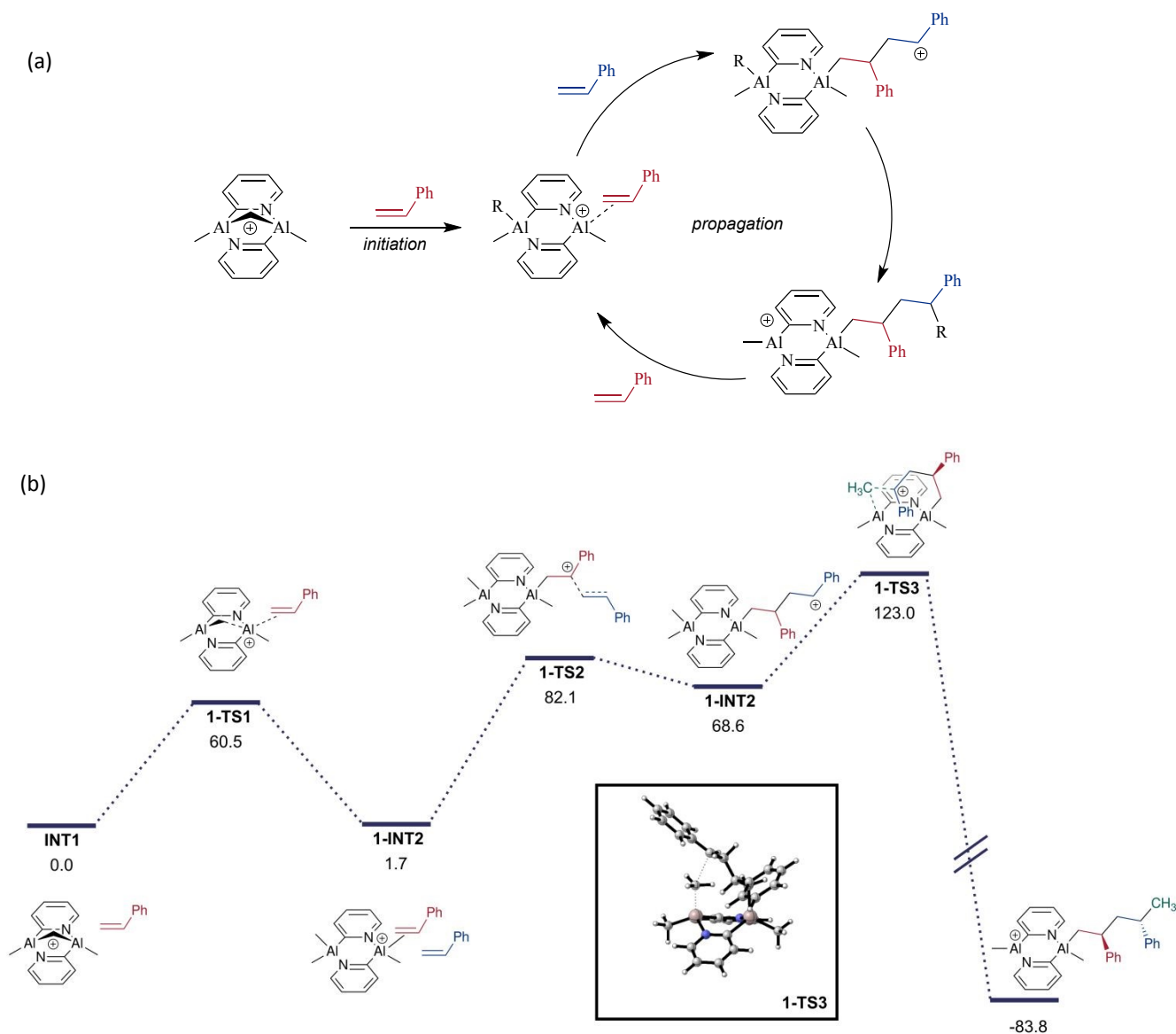
Figure 9 (a) Viable mechanism involving dimer transfer, and (b) Energy profile of the dimer transfer-based polymerisation mechanism (Gibbs free energies in kJ mol -1 ). The TS for the SE2 (back) reaction is highlighted in the box.
