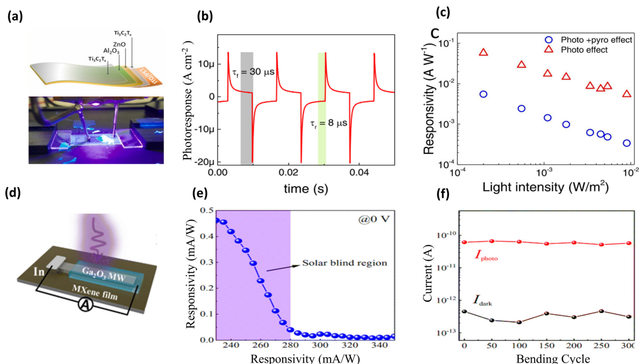
Fig. 15 (a) Schematic of the device with E- \text{Ti}_3\text{C}_2\text{T}_x and a digital image of the measurement setup, where a light wavelength of 365 nm is used, (b) Performance of the \text{Ti}_3\text{C}_2\text{T}_x/\text{Al}_2\text{O}_3/\text{ZnO}/\text{Ti}_3\text{C}_2\text{T}_x/\text{ITO}/\text{PET} TPD including photo-response speed (c) and responsivity. (d) Schematic of the \text{Ga}_2\text{O}_3 MW/MXene photodetector. (e) Photoelectric characteristics and energy band diagram of the \text{Ga}_2\text{O}_3 MW/MXene photodetector. Spectral responsivity obtained at zero bias (f) I_{\text{photo}} and I_{\text{dark}} of the device at different bending cycles (bending angles = 60^\circ ). This figure has been reproduced from ref. 215 and 216 with permission from Nano Energy, copyright 2023. CrystEngComm, copyright 2023.
