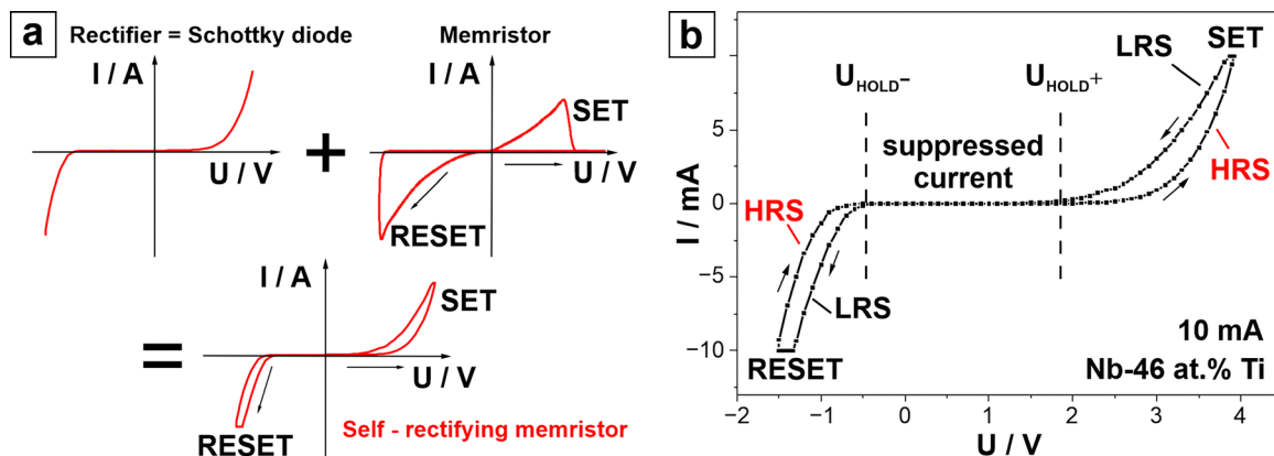
Fig. 7 (a) Typical I-U sweeps for a rectifier, a memristor and a self-rectifying memristor. (b) I-U sweep of the Nb - a 46% Ti anodic memristor. 7
