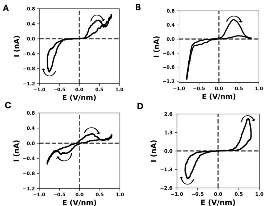
Fig. 4 I-E curves for different systems with (A) \text{Se} = -0.53e , \text{Mo} = 1.06e , \text{S} = -0.53e , (B) \text{Se} = -0.35e , \text{Mo} = 1.06e , \text{S} = -0.71e , (C) \text{Se} = 0e , \text{Mo} = 0e , \text{S} = 0e , as the membrane charges. (D) I-E curves for \text{MoS}_2 system with \text{Mo} = 1.18e , \text{S} = -0.59e as the membrane charges.
