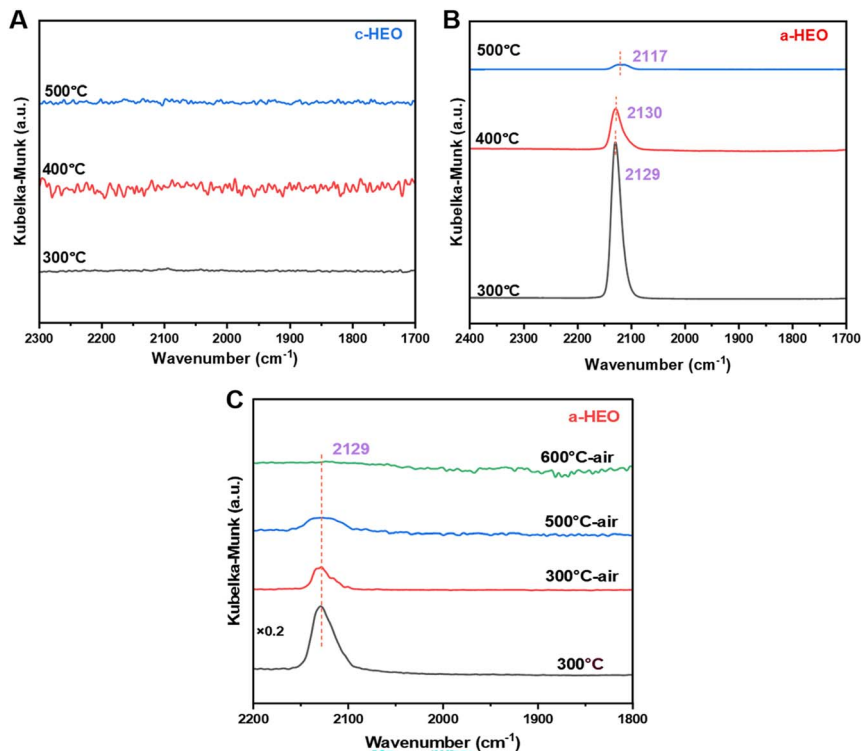
Fig. 7 CO-DRIFTS results of c-HEO (A) and a-HEO (B) at different reduction temperatures under 5% \text{H}_2/\text{Ar} atmosphere and a-HEO (C) at different oxidation temperatures under air atmosphere.
