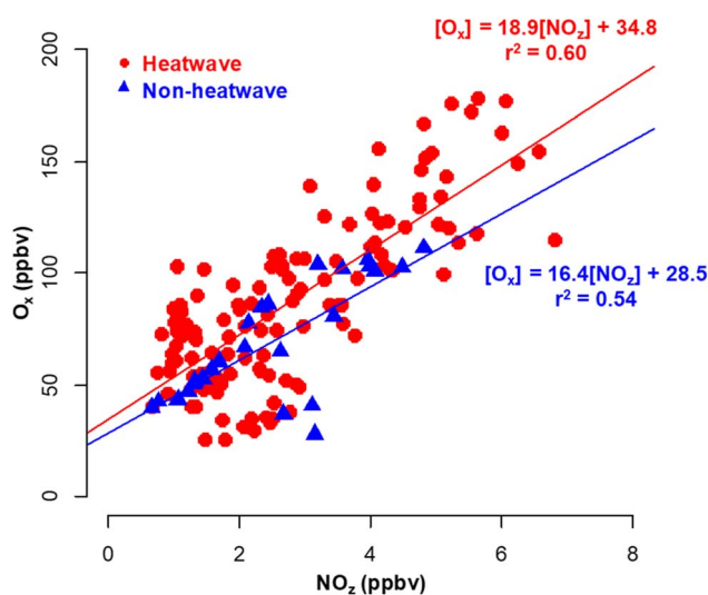
Fig. 7 The ozone production efficiency (OPE) as the ratio of O_x to NO_z during the midday (10–17 LST) for heatwave (red) and non-heatwave (blue) periods.
