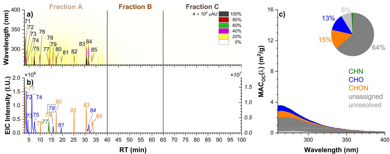
Fig. 1 Characterization of major chromophoric compounds in the DBOA sample. (a) HPLC-PDA absorbance heatmap chromatogram, (b) HPLC-HRMS extracted ion chromatogram overlay, (c) fractional MAC_{OC}(\lambda) contributions of major DBOA chromophores. Assigned PDA features are numbered in order of retention time and color-coded based on compound class. Italicized labels indicate MS features with intensities referenced to the right-hand axis; boxed labels denote BrC chromophores matched to compounds in the G1–G4 reference mixtures. Among the identified chromophores, CHON and CHN compounds contribute 16% of the total absorbance, followed by 13% contributed by CHO species.
