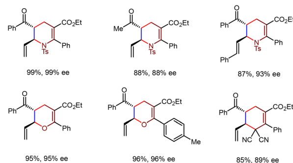
Scheme 48 Pd(0)-catalyzed asymmetric cross inverse-electron-demand [4+2] cycloadditions between 2,4-dienyl carbonyls and 1-heterodienyl/allylidenemalononitriles.
