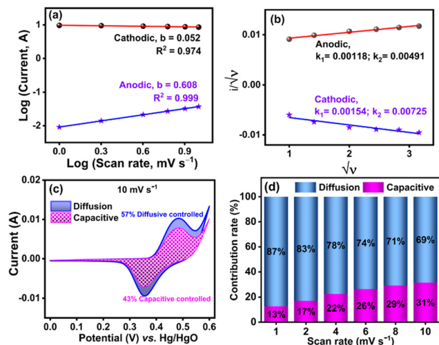
Fig. 14 Kinetics of energy storage behavior of \text{NiMoO}_4/\text{C} (D50) at different scan rates ( 1\text{--}10 \text{ mV s}^{-1} ): (a) plot of \log(i) vs. \log(v) , (b) plot of i/\sqrt{v} and \sqrt{v} , (c) CV cycles of capacitive-contribution (pink-shaded region) and diffusion-contribution (blue-shaded region) at 10 \text{ mV s}^{-1} , and (d) total contribution rate of capacitive (pink) and diffusion-controlled (blue) processes at different scan rates.
