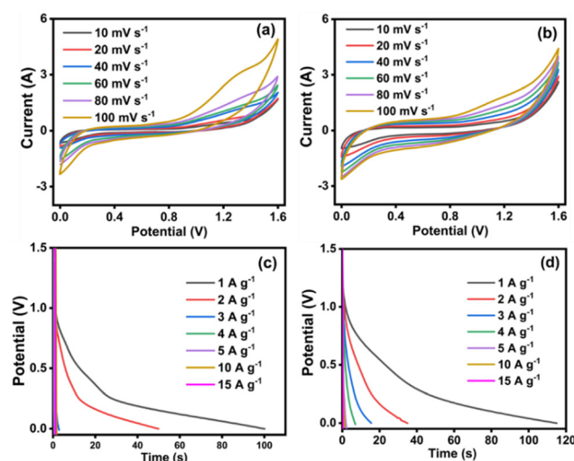
Fig. 15 The electrochemical performances of \text{NiMoO}_4/\text{C} (D50) based symmetric (left) and asymmetric (right) SCs: (a) and (b) CV curves at different scan rates, and (c) and (d) GCD curves at different current densities.
