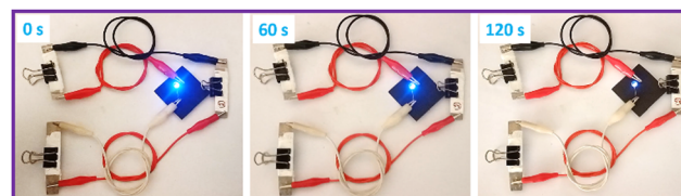
Fig. 16 Demonstration of powering a blue LED light by three \text{NiMoO}_4/\text{C} (D50) based symmetric SC devices connected in series.
