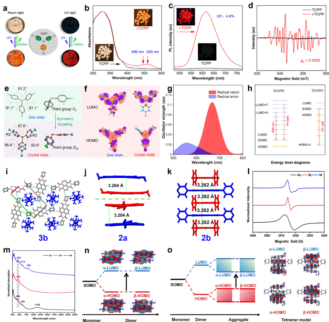
Fig. 3 Photoinduced stable radical generation and luminescence. (a) Schematic illustration of the reversible photochromic transformation of TCPP crystals into emissive radical cations under UV light, exhibiting red luminescence upon irradiation and recovering under visible light. The molecular structure of TCPP is shown centrally. (b) UV-vis absorption spectra of TCPP crystals before and after UV exposure ( \lambda_{\text{ex}} = 365 nm), with insets showing the corresponding appearance changes. (c) PL spectra of neutral and UV-activated TCPP (i-TCPP) crystals; quantum yield (QY) of the radical emission is 4.6%. Insets: Fluorescence photographs under UV excitation. (d) Electron paramagnetic resonance (EPR) spectra reveal a strong radical signal at g_e = 2.0035 for i-TCPP. (e) Comparison of the ground-state molecular geometries of TCPP in the gas phase and crystal phase, highlighting symmetry breaking from C_3 to D_{2h} due to intermolecular packing (DFT, BLYP/def2-SVP). (f) TD-DFT-calculated HOMO and LUMO orbitals of TCPP in gas and crystal states (M062X/def2-TZVP), showing enhanced charge delocalization in the crystal state. (g) Simulated oscillator strengths of radical cation and anion emissions (PBE0/def2-TZVP). (h) Frontier molecular orbital energy diagrams of the TCPP radical cation and anion (M062X/def2-TZVP), illustrating spin-orbital distributions in the excited state. Reproduced with permission from ref. 86. Copyright © 2021, Chinese Chemical Society. (i) Crystal packing diagram of radical 3b. (j) Side views of pairs of radical 2a viewed along the direction parallel to molecular long axis and short axis. (k) 1D \pi -stacking in 2b crystals, featuring a uniform intermolecular separation of 3.262 Å. (l) EPR spectra of 2a, 2b, and 3b radicals, indicating varying spin densities and packing effects. (m) Solid-state UV-vis-NIR absorption spectra of 2a, 2b, and 3b crystals embedded in KBr, showing distinct long-wavelength absorption features. (n) and (o) Schematic diagrams of SOMO-to-LUMO excitation in a 2a dimer (n) and 2b tetramer aggregate (o), based on UMN15/def2-TZVP calculations. Energy levels and spatial distributions of \alpha/\beta HOMO and LUMO orbitals are shown. Reproduced with permission from ref. 58. Copyright © 2025, Chinese Chemical Society.
